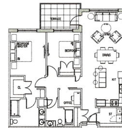
UNIT G 2-BEDROOM 1234sf ESTATE
